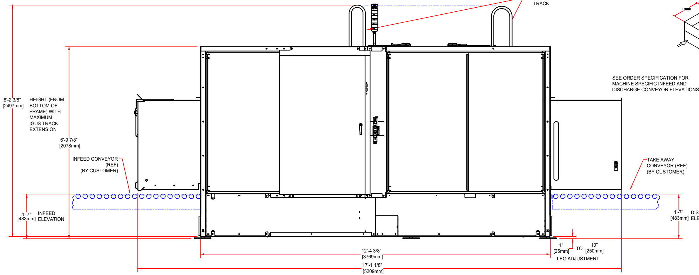
ELEVATION VIEW
