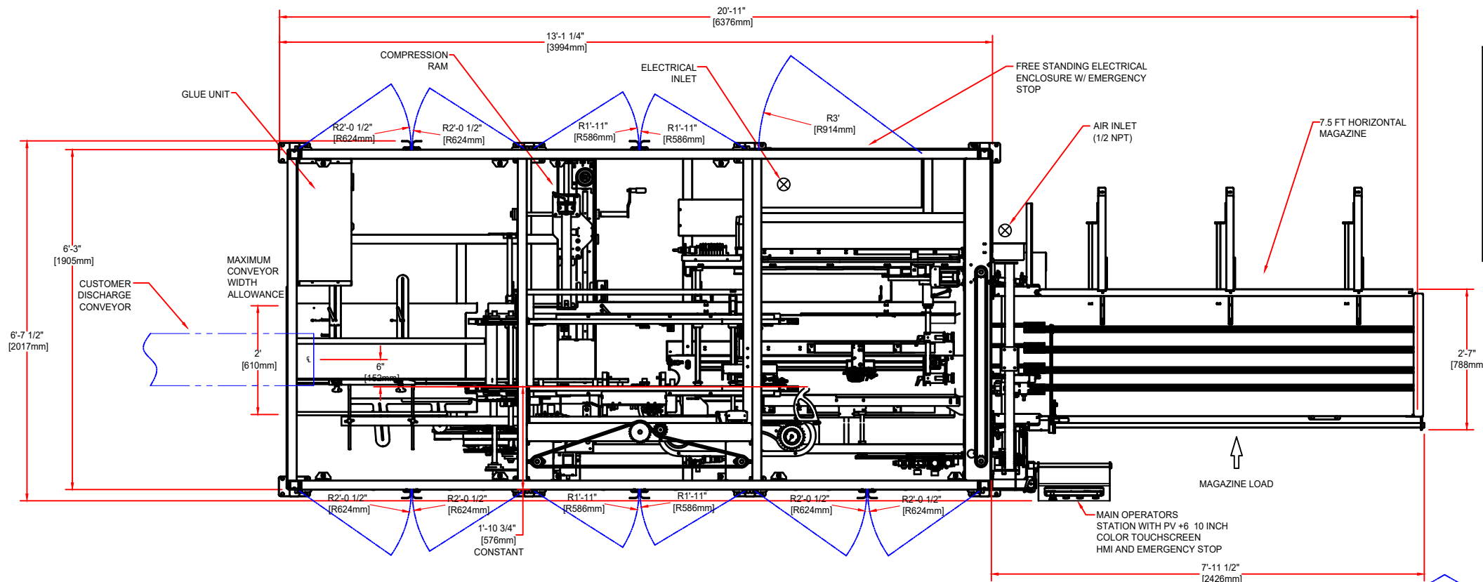
PLAN VIEW
