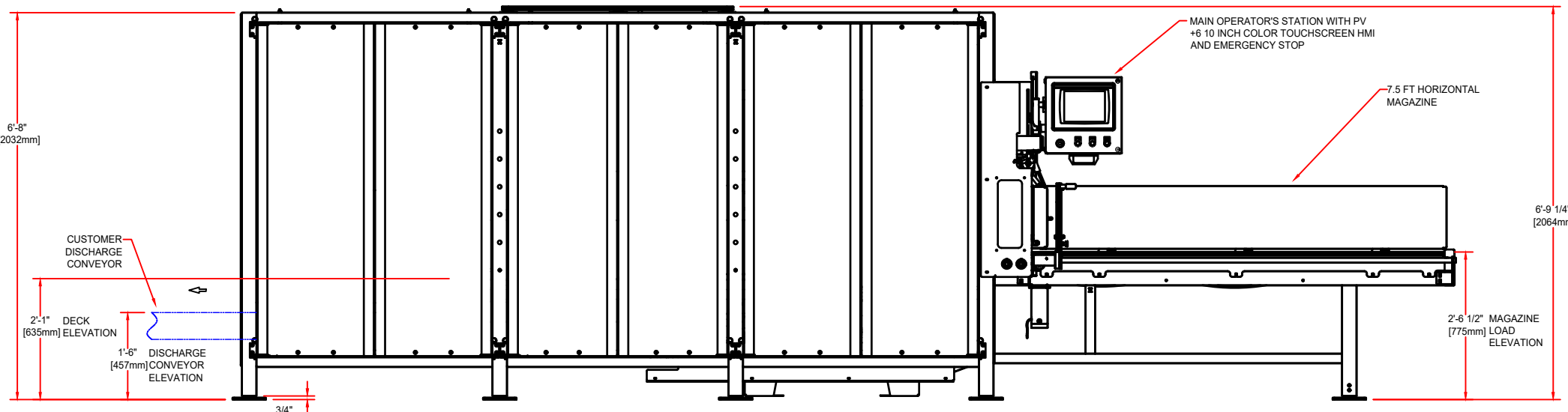
ELEVATION VIEW
