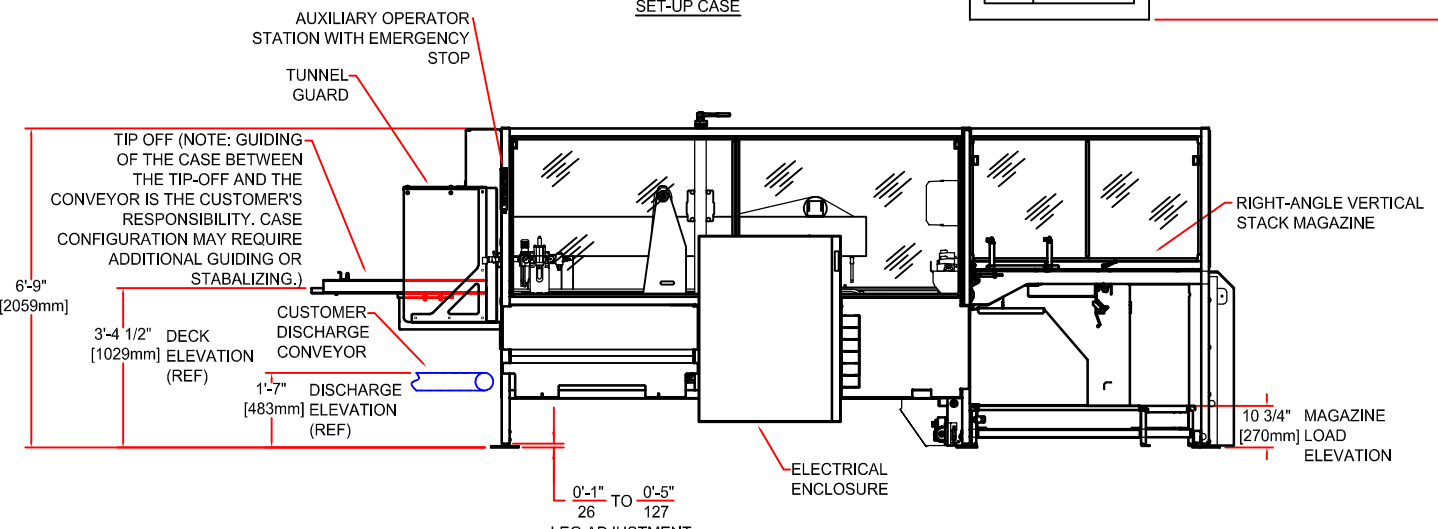
ELEVATION VIEW
